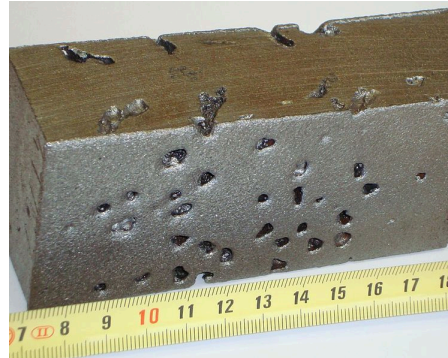
Gasporosität in GS-20Mn5 - Gussstahl at wikipedia - CC-BY-SA 3.0
